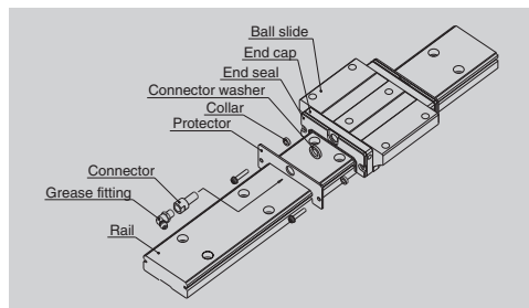
Fig. 11 Protector seal
