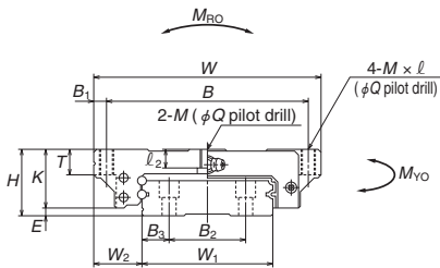
Front view of EL types
