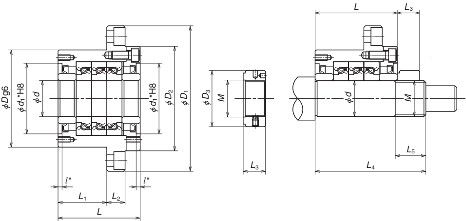
Lock nut
