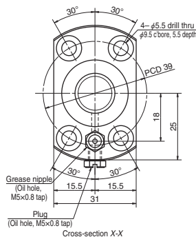
Cross-section X-X
