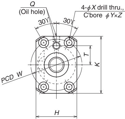
View X-X
