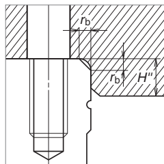
Fig. 11 Shoulder for the roller slide datum face
