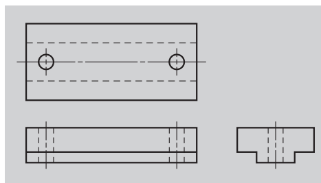
Fig. 2 Fitting plate
