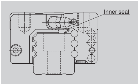
Fig. 6.6 Inner seal when installed
