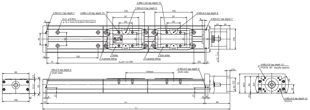
Dimension of MCH10 (Double slider)
