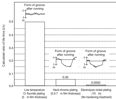
Fig. 3.1 Result of durability test
