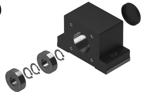
Pillow block unit SES-L assembly
