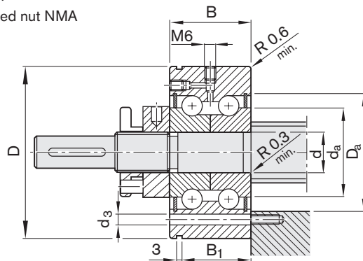
LGF-C-... with slotted nut NMA
