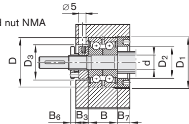
LGN-B-... with slotted nut NMA
