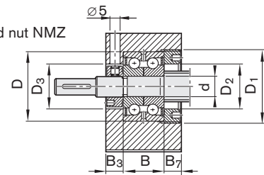
LGN-B-... with slotted nut NMZ
