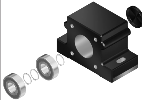
Pillow block unit SEC-L assembly
