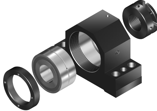
Pillow block unit SEB-F assembly
