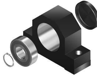
Pillow block unit SEB-L assembly
