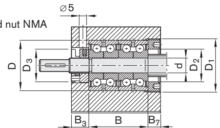
LGN-C-... with slotted nut NMA
